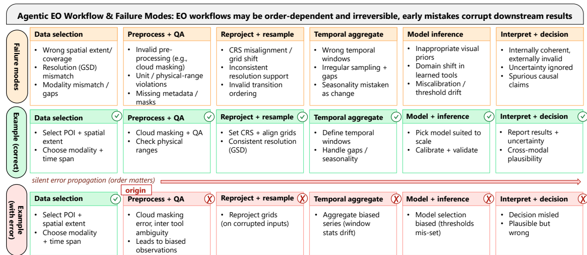
Fig. 5. Agentic EO workflow and representative failure modes. The figure illustrates how errors introduced during data selection, preprocessing, reprojection, temporal aggregation, or model inference can propagate through downstream analytical stages. It also contrasts a geo-valid workflow with an error-prone workflow to highlight how early mistakes may silently corrupt later decisions.
