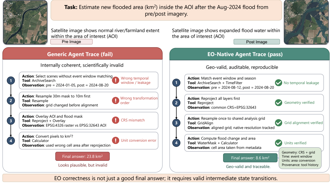
Fig. 2. Illustrative comparison of generic and EO-native agent traces for flood-area estimation from pre/post imagery. The generic trace reaches a plausible-looking but invalid result because the workflow contains representative EO failure modes, including temporal-window mismatch, incorrect transformation order, coordinate reference system (CRS) mismatch, and unit-conversion error. The EO-native trace illustrates the corresponding valid workflow: matching the event window, reprojecting layers to a common CRS, aligning data to a shared analysis grid, and computing area using metadata. The example highlights that EO correctness depends not only on the final answer, but also on valid intermediate state transitions. Figure developed with the help of ChatGPT.
