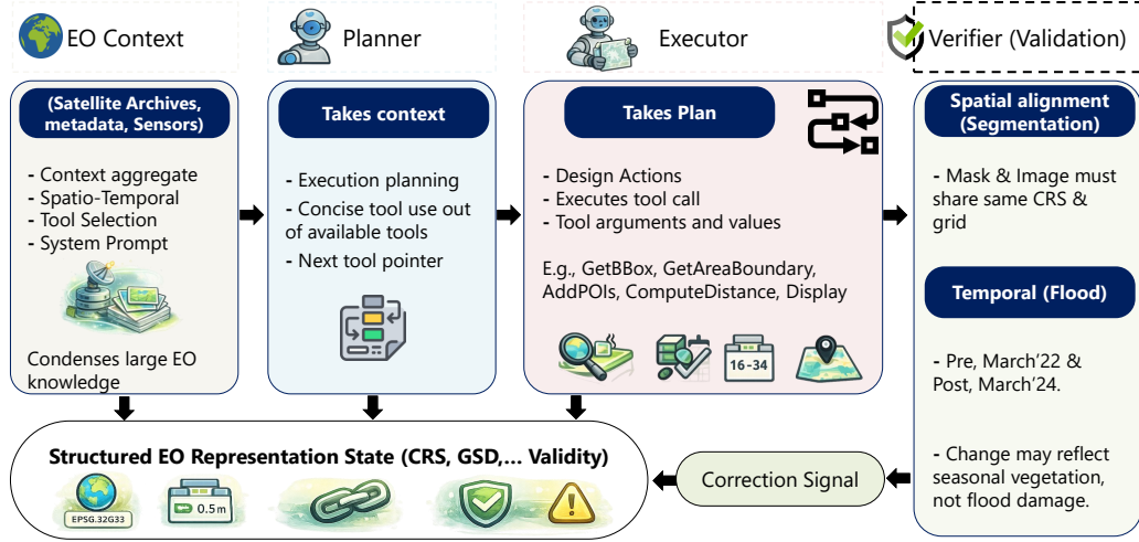
Fig. 7. Design blueprint for agentic Earth observation. This consists of a Planner, Executor, and Verifier operating over a shared structured EO state representation. The Planner condenses large EO context into an execution plan, the Executor performs tool calls with explicit arguments, and the Verifier ensures geospatial and physical validity through checks such as CRS consistency, spatial alignment, temporal validity, and physically meaningful interpretation (e.g., distinguishing seasonal vegetation change from flood damage). Drawings from ChatGPT.
