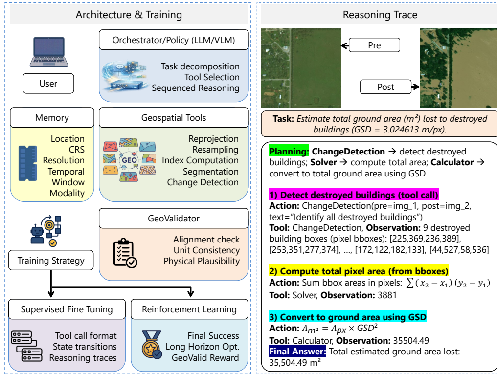
Fig. 6. Agentic EO architecture and tool-integrated reasoning. Left: The agentic model includes an orchestrator policy (LLM/VLM), structured memory, geospatial tools, and a GeoValidator for enforcing spatial consistency. Training combines supervised fine-tuning and reinforcement learning with geospatial validity rewards. Right: Example reasoning trace showing sequential tool usage to estimate ground area lost to destroyed buildings from pre/post imagery using change detection and GSD-based area conversion. Drawings from ChatGPT.
