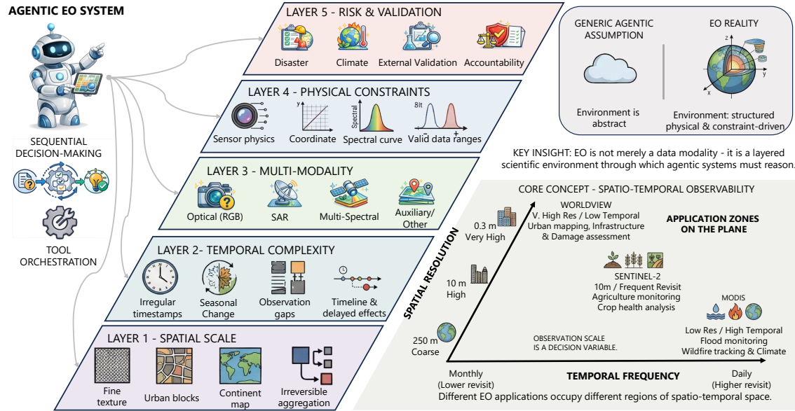
Fig. 4. Structural properties of Earth observation environments for agentic models. EO reasoning operates within a layered environment characterized by spatial scale, temporal complexity, multi-modality, physical constraints, and risk-aware validation. These layers jointly define the conditions under which agentic EO models must perform sequential decision-making and tool orchestration. The figure also illustrates spatio-temporal observability, where different EO applications occupy distinct regions of the spatial-resolution and revisit-frequency space, making observation scale a critical decision variable for agentic reasoning. The sensing sources shown are representative rather than exhaustive. Figure developed with the help of ChatGPT.
