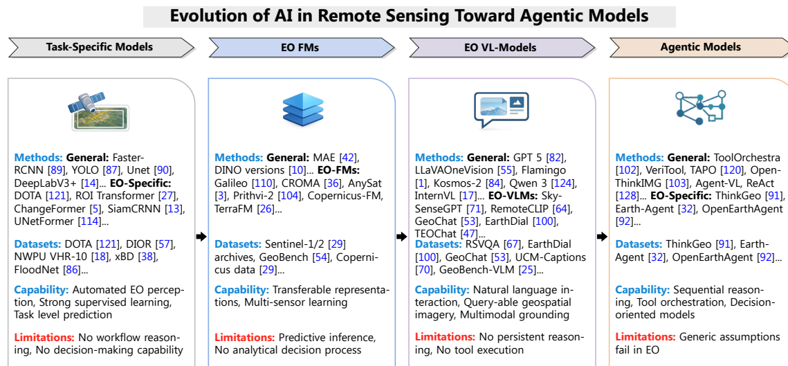
Fig. 1. Evolution of AI paradigms in remote sensing toward agentic models. The field has progressed from task-specific predictive models to EO foundation models, EO vision-language models, and emerging agentic frameworks. Each stage expands the capability space from automated perception and transferable representation learning to language-grounded interaction and sequential tool use. At the same time, this progression exposes a mismatch between generic agentic assumptions and EO workflow constraints, motivating agentic models that reason over geospatial state, tool effects, and validity rather than final predictions alone. Drawings from ChatGPT.
